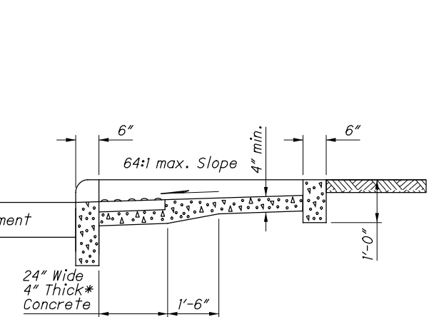
SECTION C-C See Sheet 2.
