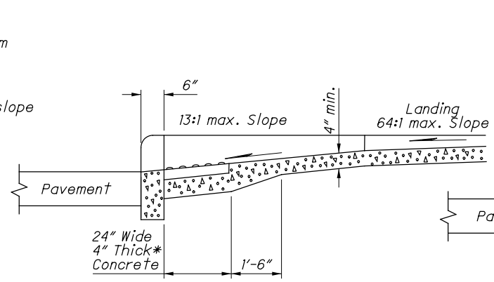
SECTION B-B See Sheet 2.
