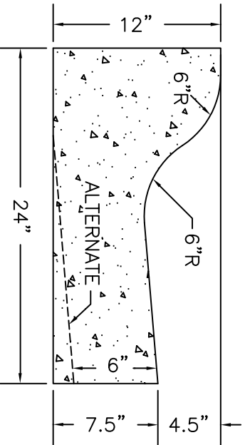
COMBINATION CURB & GUTTER TYPE 'C'
