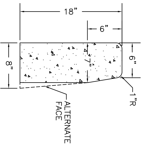
CURB-TYPE 'A'
